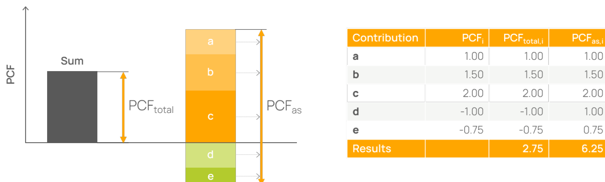
1148 1149 Figure 14: Definition of PCF_{as} : a-e represent contributions to the PCF; d and e are biogenic CO 2
